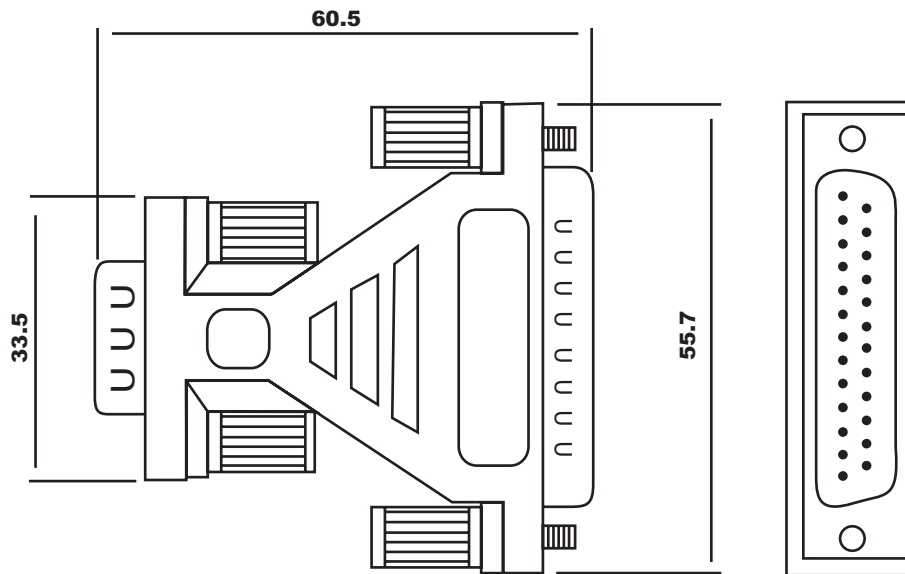
P2 Moulded
